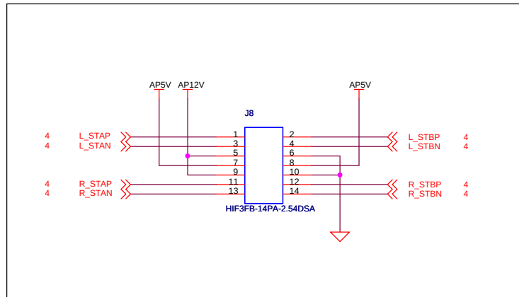
STEP MOTOR
