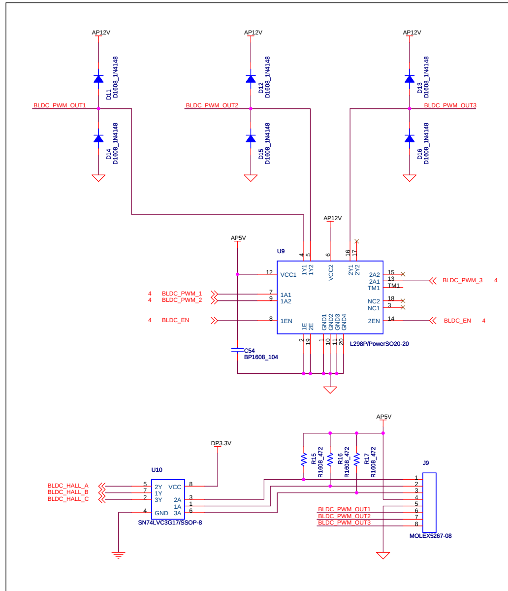
BLDC MOTOR DRIVER
